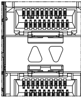
TYPE3_INNER LIGHT PIPE 1073222CF001 1073222CF002
