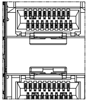
TYPE1_NONE LIGHT PIPE 1073202CF001 1073202CF002
