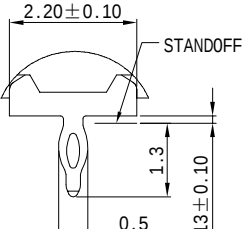
DETAIL PIN3 SCALE 10:1
