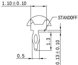
DETAIL PIN1 SCALE 10:1
